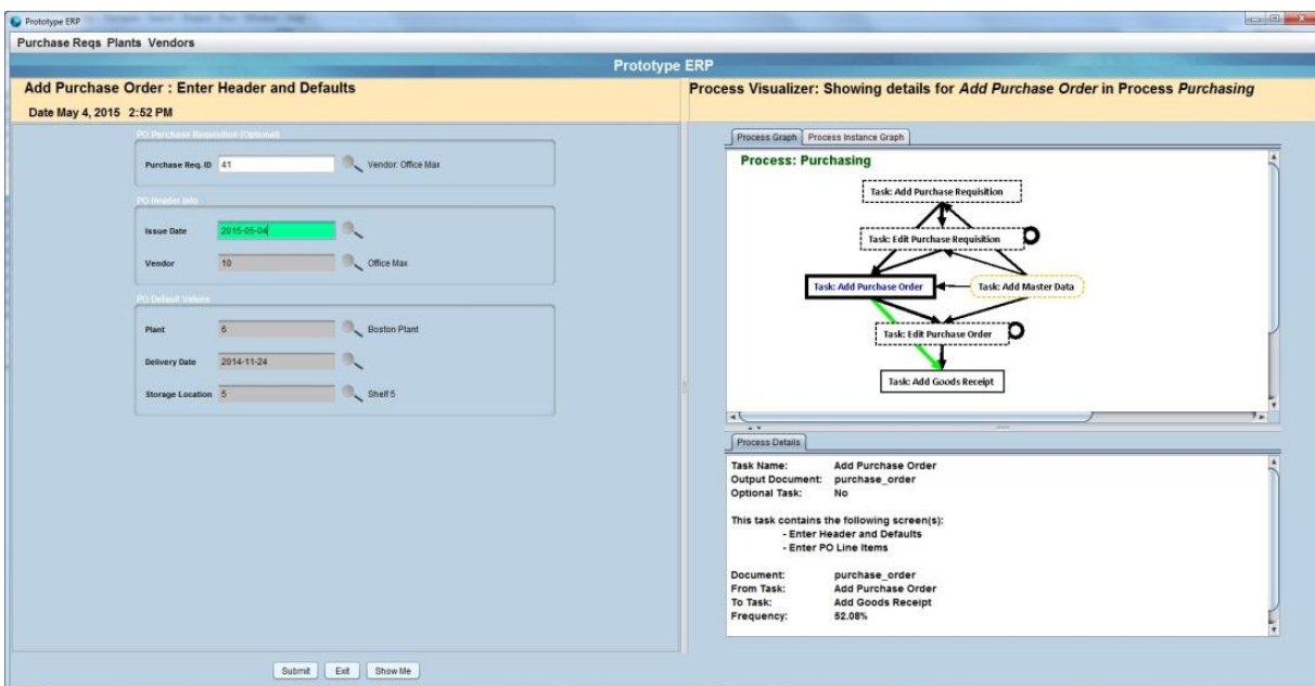
(a) ERP prototype with the Interactive Process Visualization component on the right
