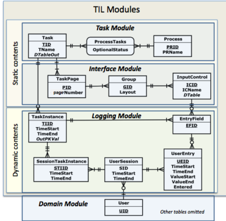
Figure 4: The Entity-Relationship diagram of the TIL model (figure from an earlier paper)
