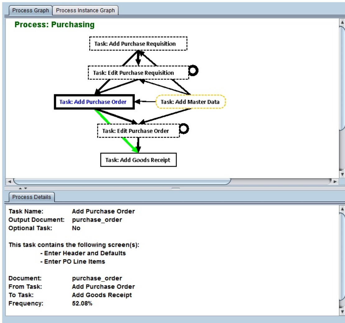
(b) Enlarged fragment of Figure 6a, showing the Process Graph and Process Details panes of the Interactive Process Visualization
