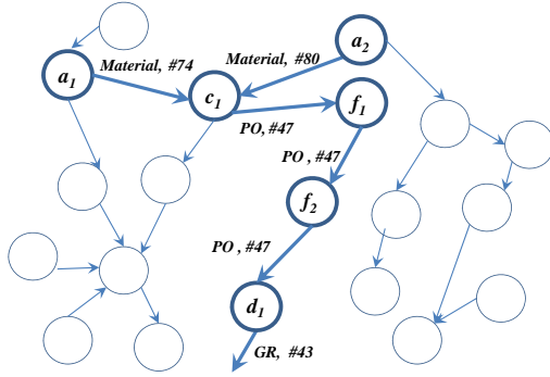
Figure 3: A fragment of a task instance graph with a process instance highlighted in boldface.
